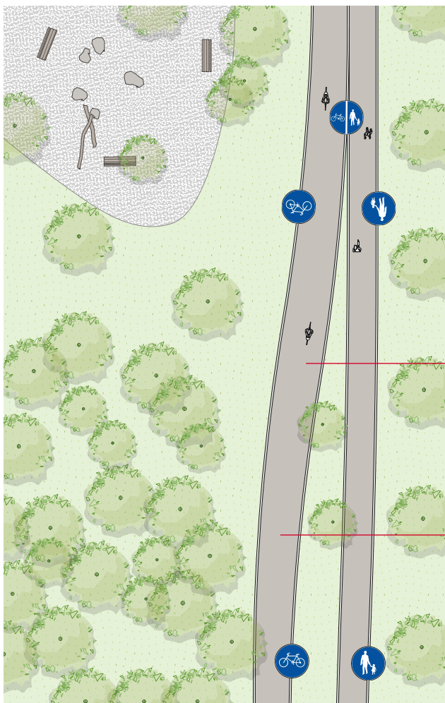
Situationsplan (1:500)
